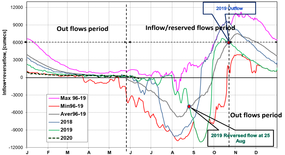
Figure 4 The seasonal change of inflows and outflows of the Tole Sap Lake
